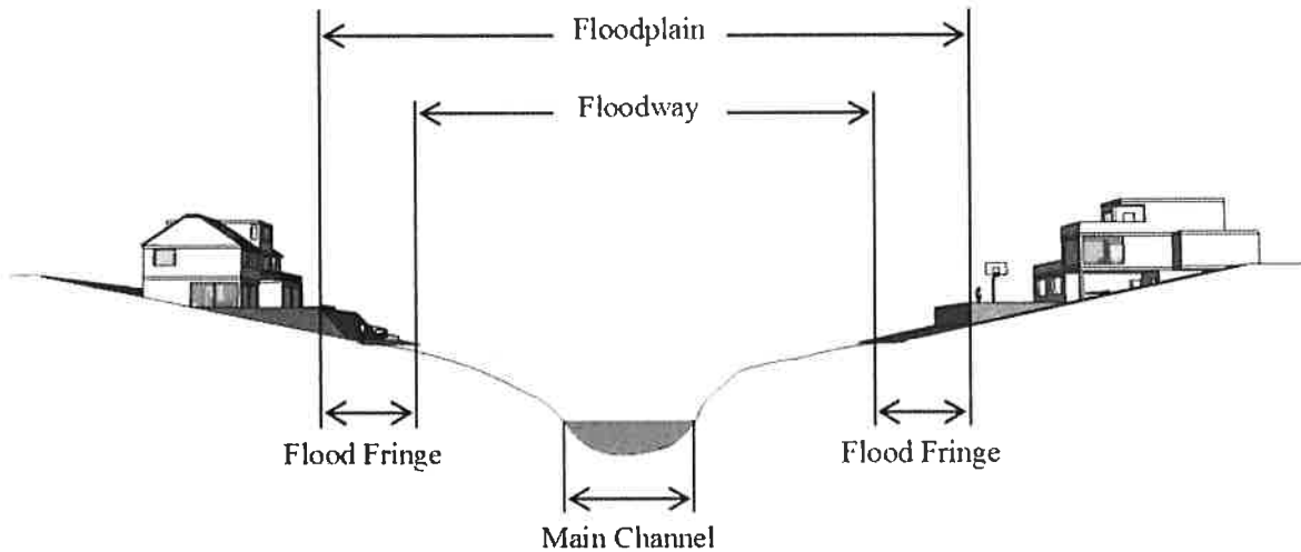
FIGURE 5: CROSS-SECTION OF A FLOOD FRINGE AND FLOODPLAIN
